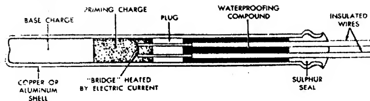
ELECTRIC BLASTING CAP
